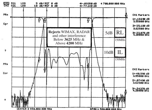
11383-3625/4200 Typical Response
