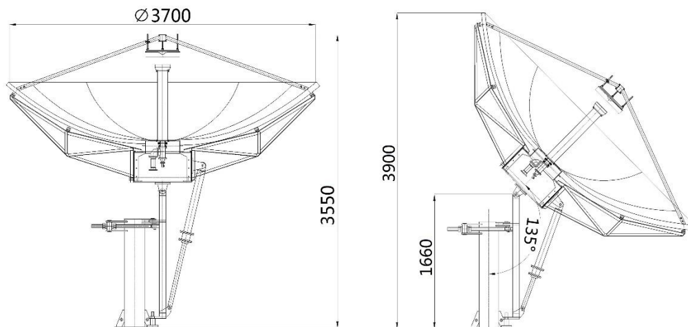
Mechanical Diagram (Unit: inch (mm))
