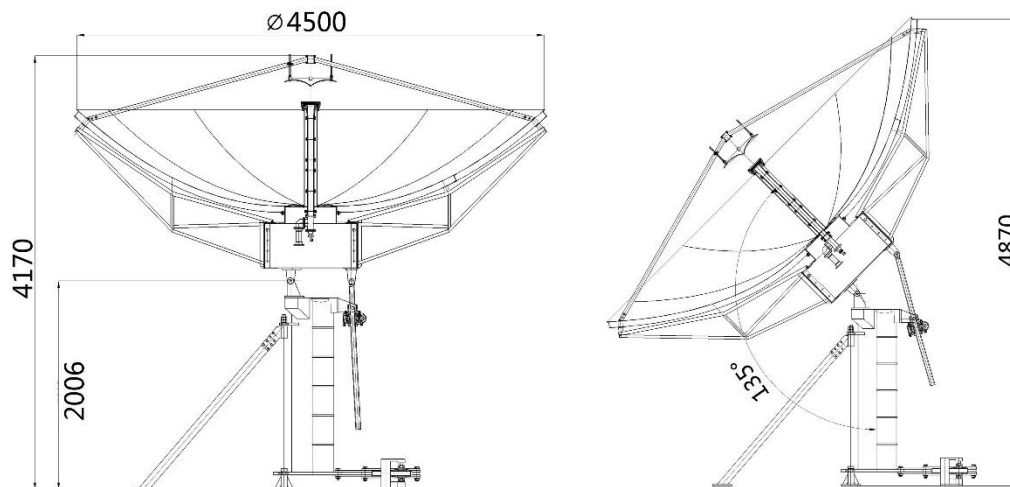
Mechanical Diagram (Unit: inch (mm))
